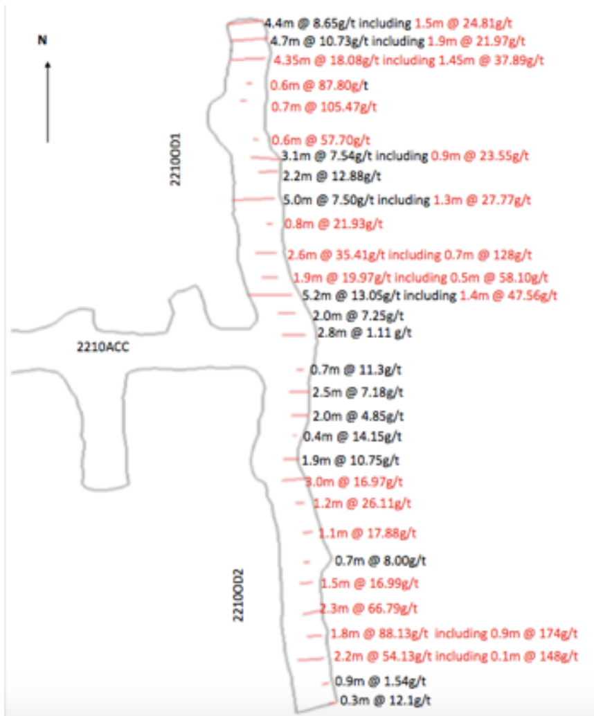
2210 level showing face by face uncut gold assay grade. Grades exceeding 15 g/t Au are highlighted in red.
